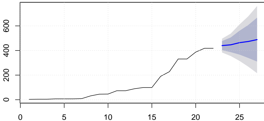
Figure 7: ARIMA projection
